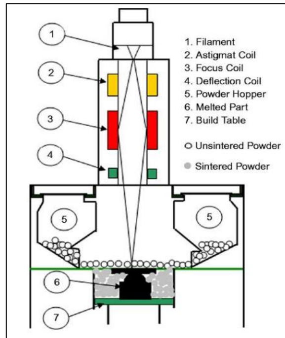
Figure 4: Electron Beam Melting (Courtesy of Manuela Galati et.al. [14])
